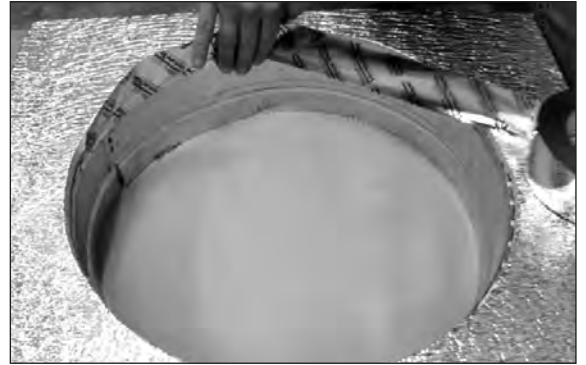
10. Put the insulation to the inner side of the panel and fix the insulation to the collar with a duct tape.
